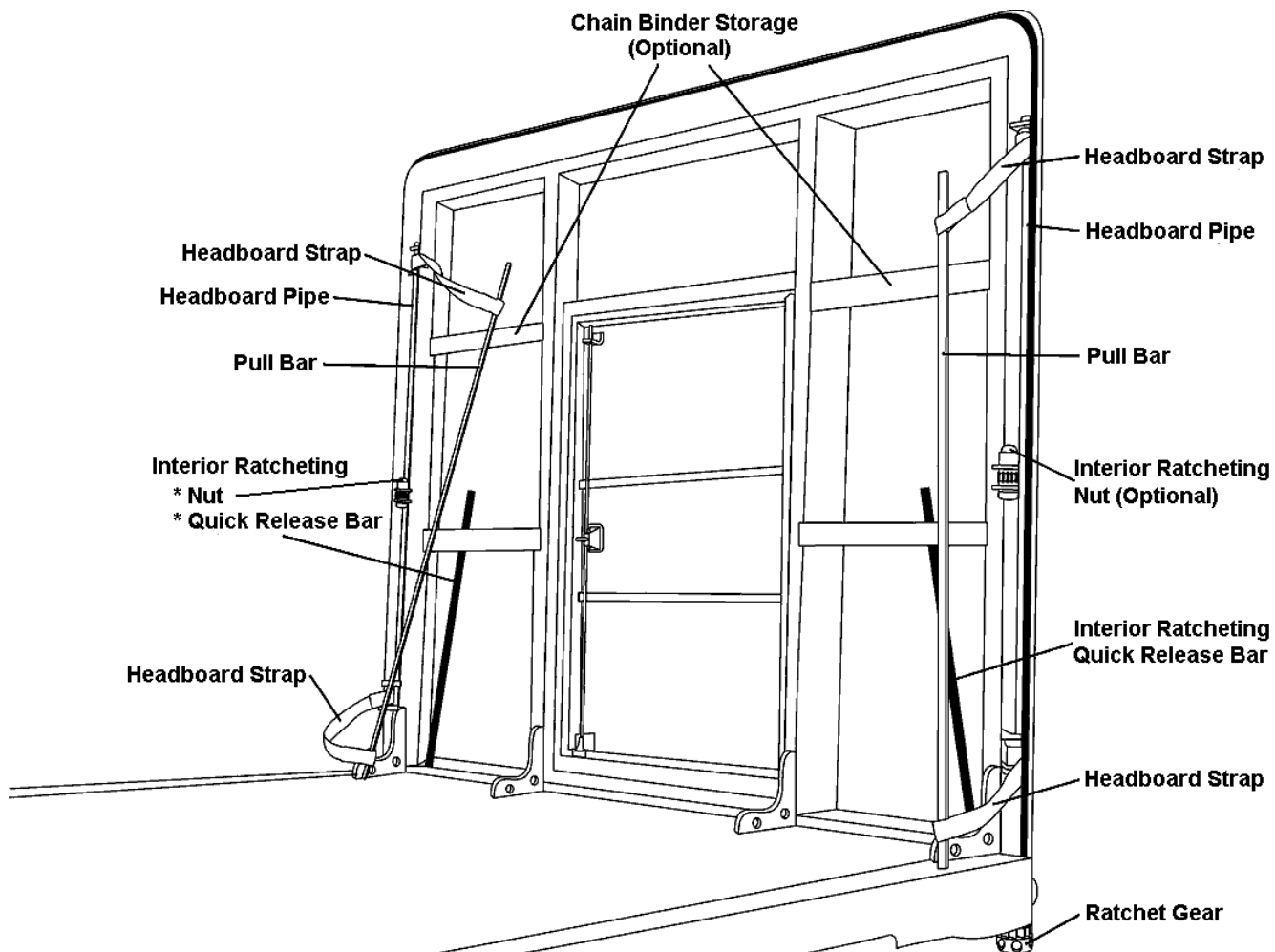
F.01.B: Component naming reference: Headboard inside view
